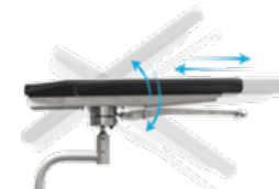
Armrest pair with linear guide and one-hand release, adjustment range 110 mm, factory-fitted
