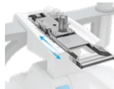
Seat adjustment mechanism for optimum access to the operating field, adjustment 113 mm, factory-fitted
